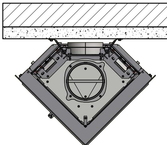
Fastmontering parallell
